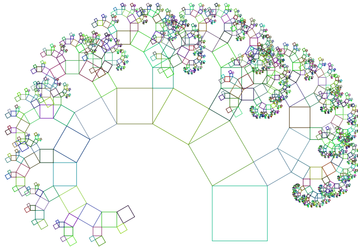
Pythagoras Tree, order 11, angle 65:
