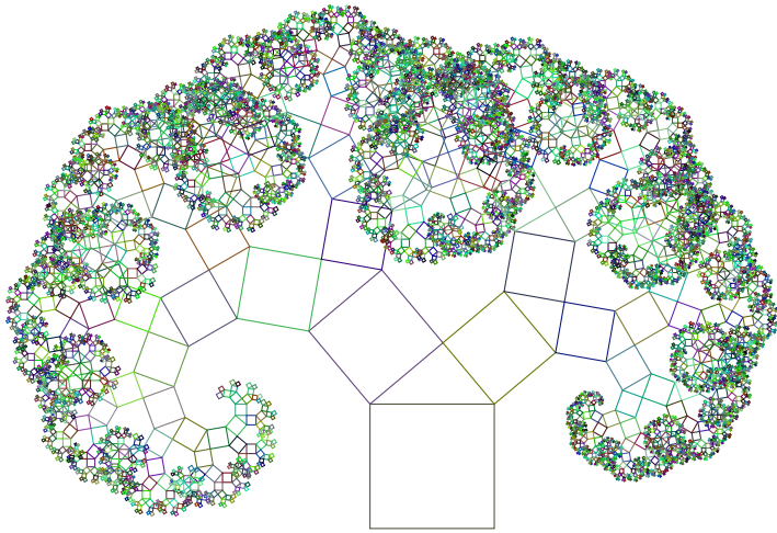
Pythagoras Tree, order 13, angle 38:
