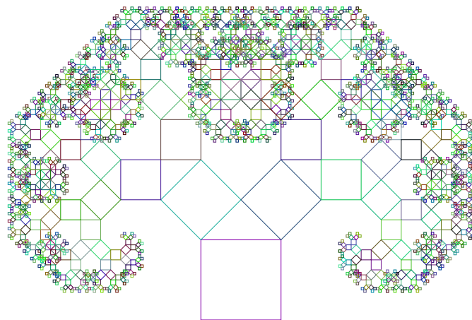
Pythagoras Tree, order 11, angle 45:
