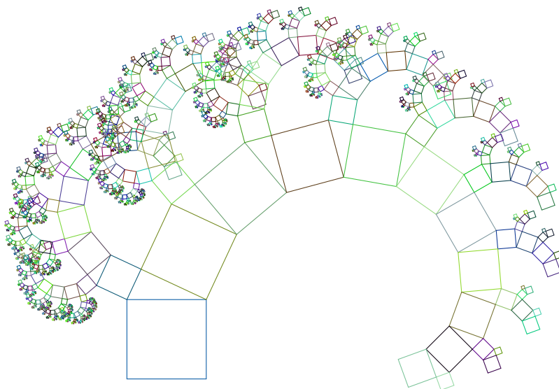
Pythagoras Tree, order 11, angle 65:
